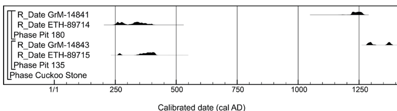
Figure 4: Probability distribution of the dates on carbonised cereal grains from the Cuckoo Stone. The distributions are the result of simple radiocarbon calibration (Stuiver and Reimer 1993)
