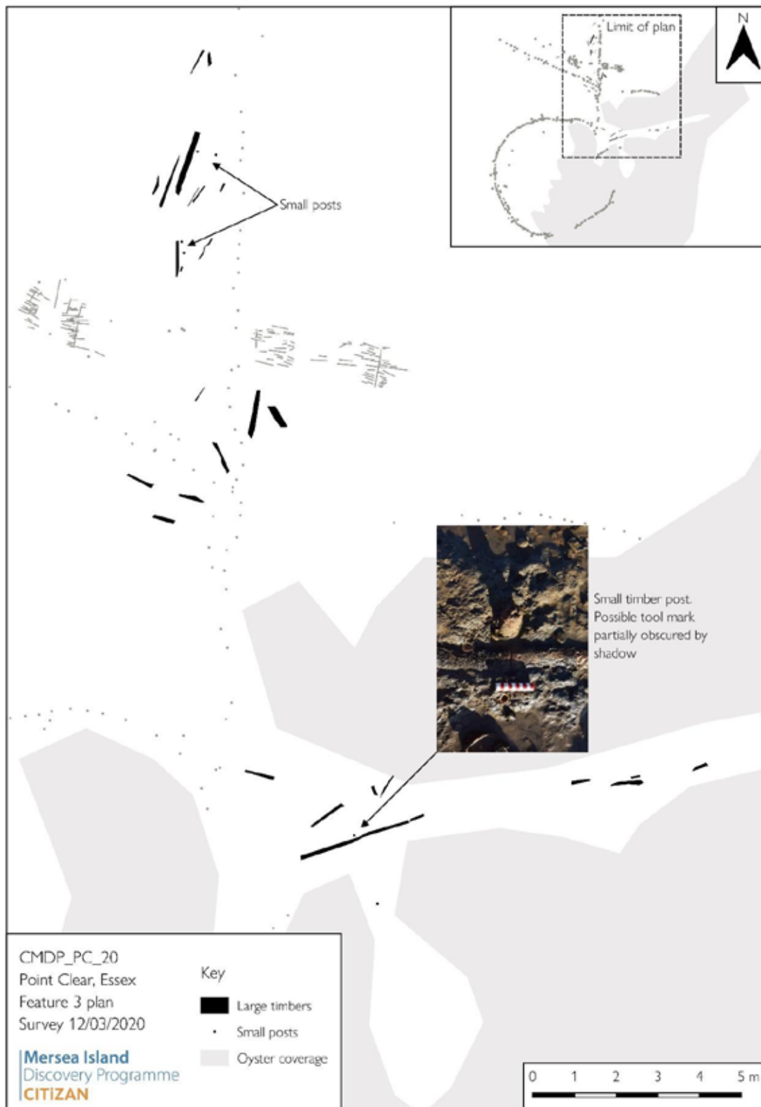
Figure 8: Feature group 3 (© O Hutchinson).
