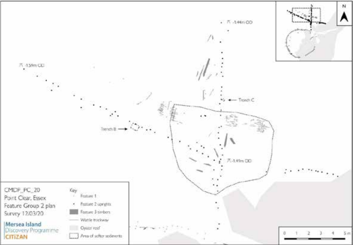
Figure 5: Feature group 2 (© O Hutchinson).
