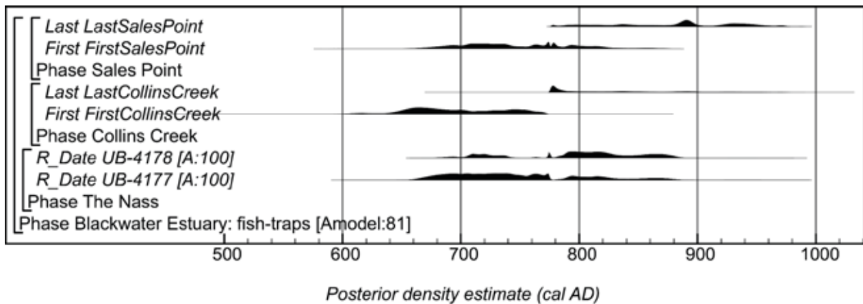
Figure 16: Probability distributions of dates for the construction of fish-traps in the Blackwater Estuary derived from the model described in Appendix 2 (Fig. 17) (© Historic England).
