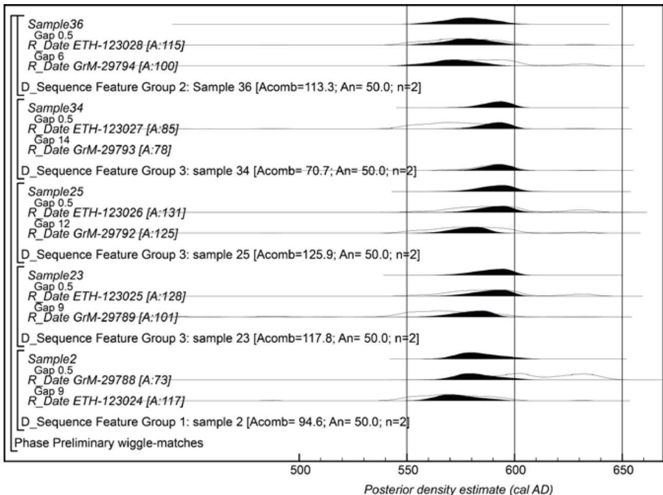
Figure 11: Probability distributions of dates from Point Clear: wiggle-matches.
