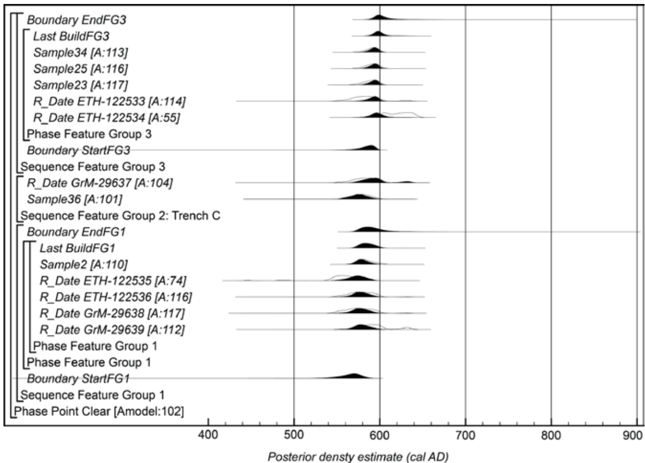
Figure 12: Probability distributions of dates from Point Clear.
