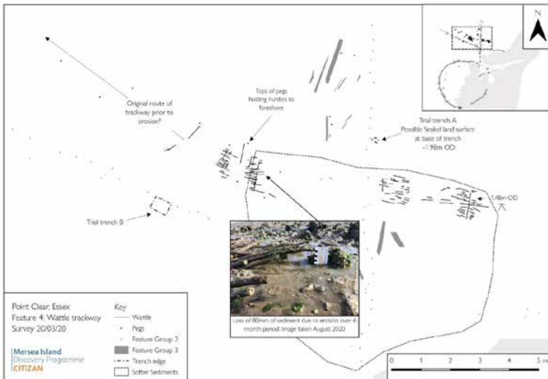
Figure 9: Feature group 4 (© O Hutchinson).
