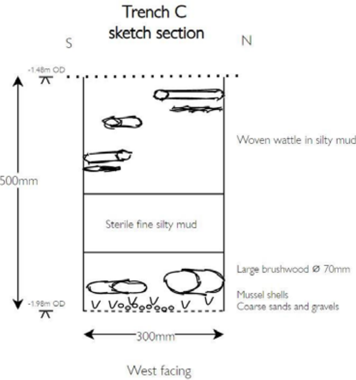
Figure 6: Trench C sketch section (© O Hutchinson).
