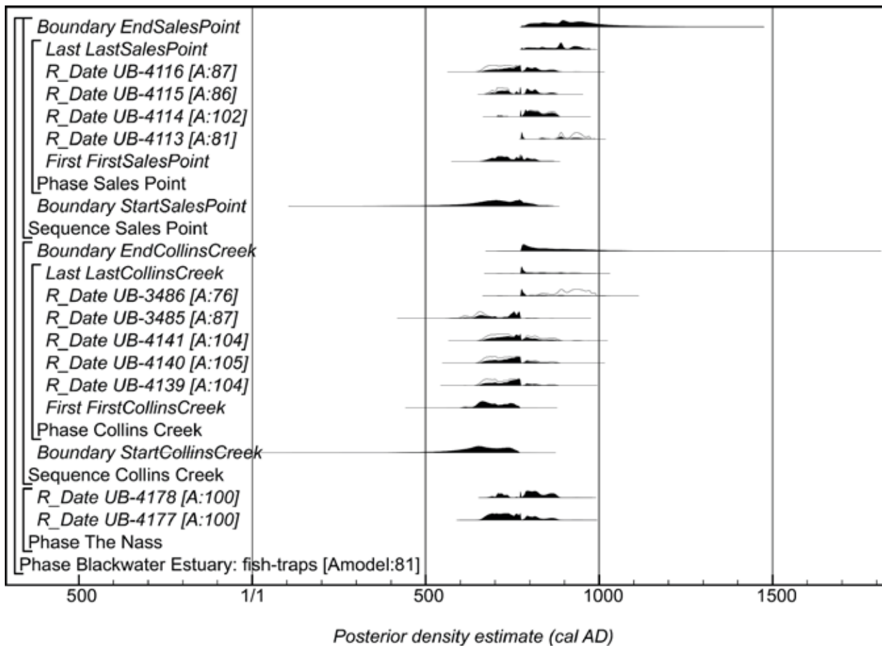
Figure 17: Probability distributions of dates from Blackwater Estuary fish-traps: The Nass, Collins Creek and Sales Point. The format is identical to Figure 12 (© Historic England).
