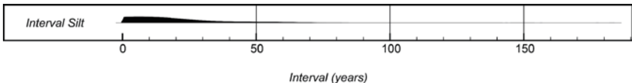
Figure 13: Probability distribution for the number of years it took the silt deposit in Trench C (Feature group 2) to accumulate, derived from the model defined in Figure 12.
