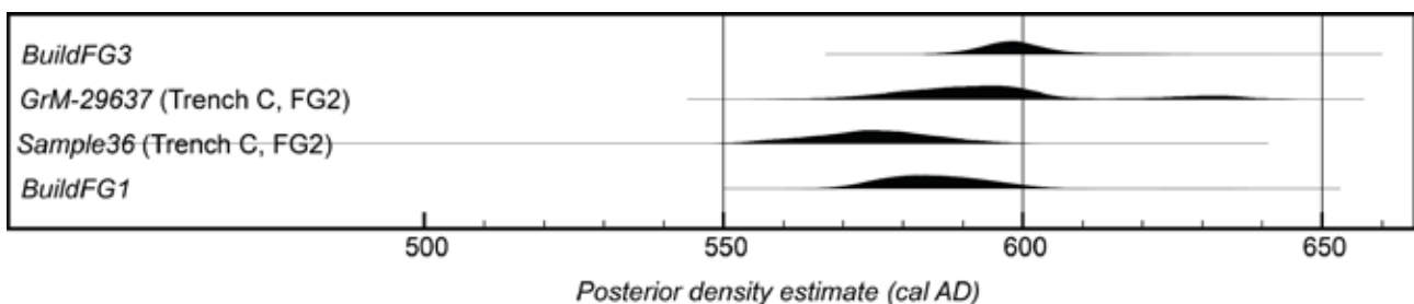
Figure 14: Probability distributions of dates for the construction of wooden structures at Point Clear, derived from the model defined in Figure 12.
